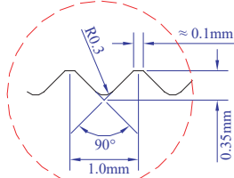
GROOVE DETAIL
